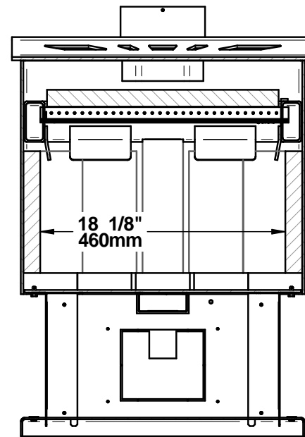
SECTION B-B
